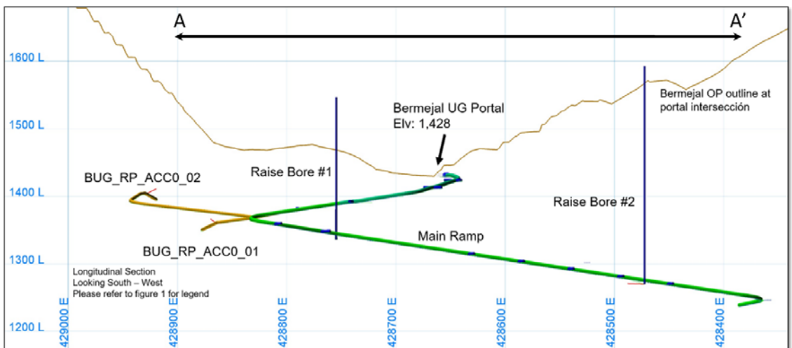
Figure 2: Vertical Longitudinal Section of Bermejaj Underground Development
